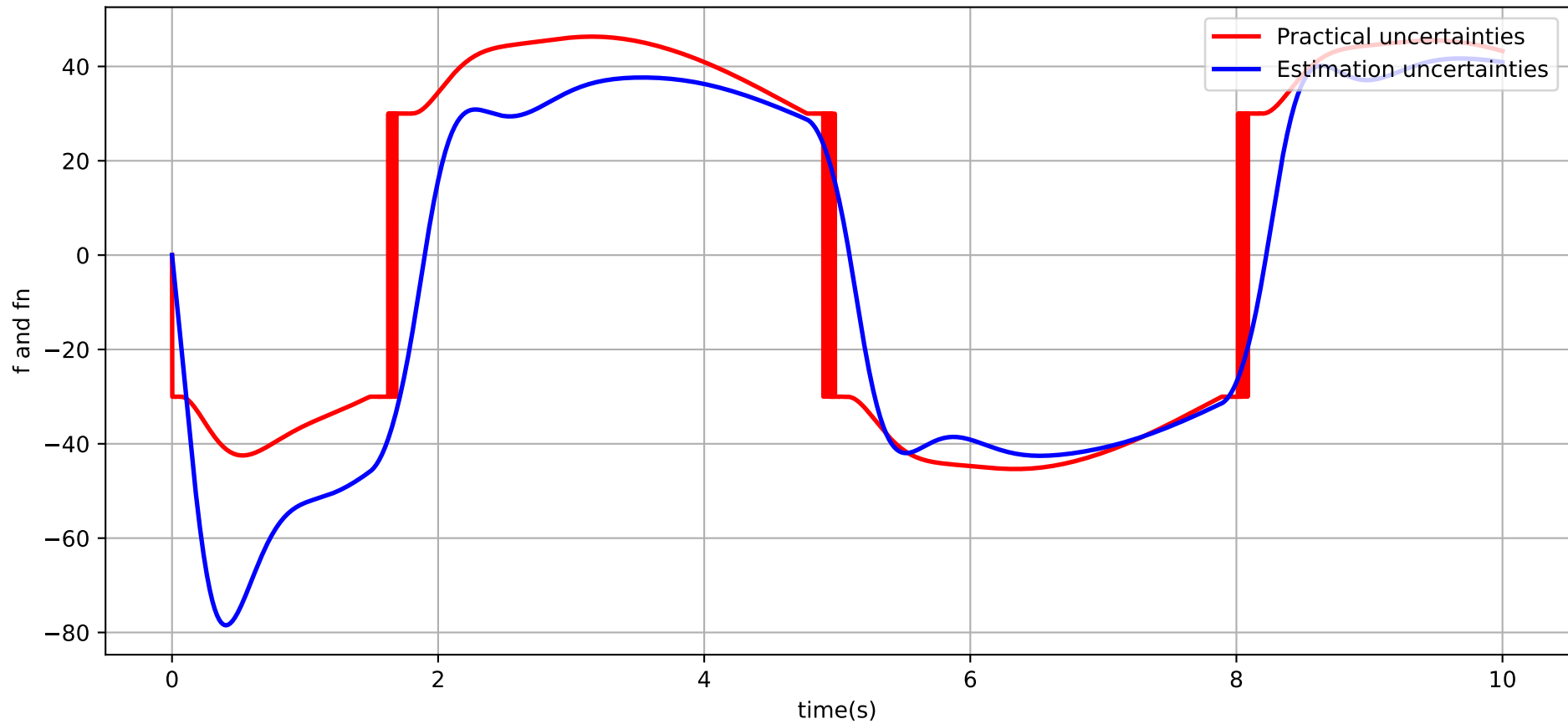
Disturbance Estimation Performance ( S=3 , S1=2 , m=5 )
